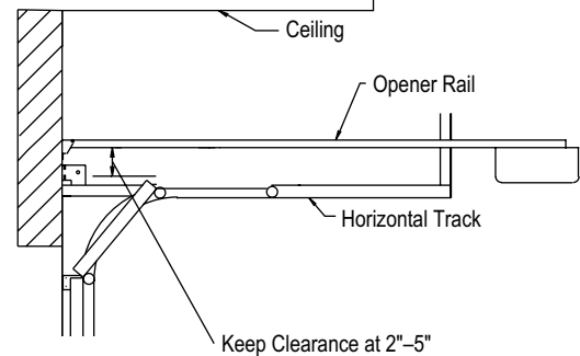
Opener Rail Mounting Distance
