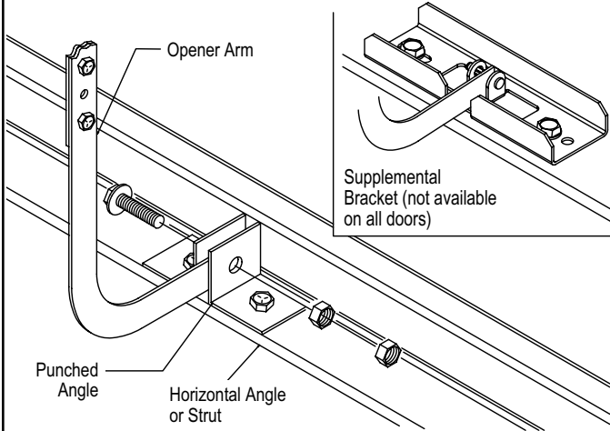
Front View (assembled)
