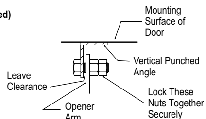
Fig. 15-D (Doors with angle iron reinforcement bracket and stile in center of door)
