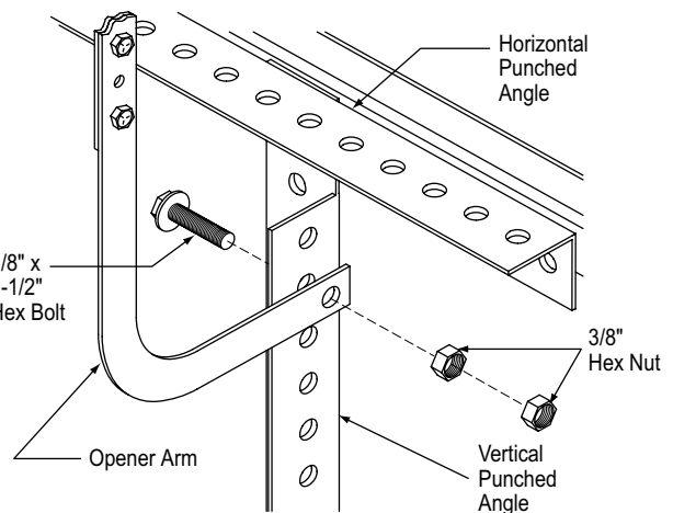
Top View (assembled)
